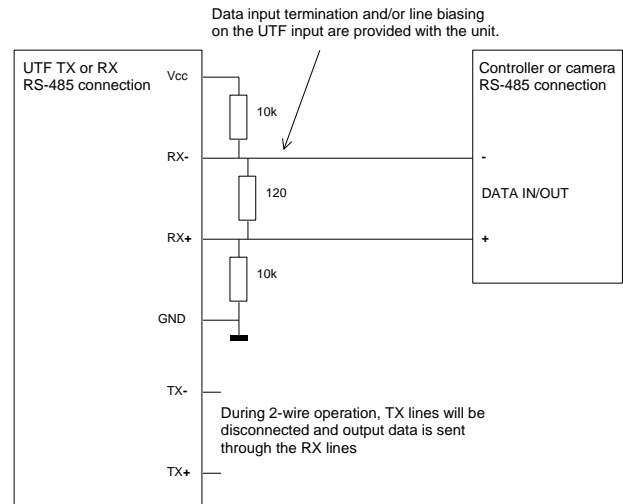
Figure 6. 2-Wire connection
