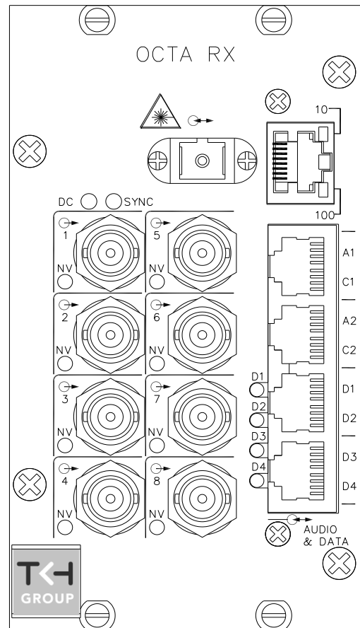
Figure 1. OCTA 43x0 RX front panel, TX panels look similar, with video inputs instead of outputs (see table 1).
