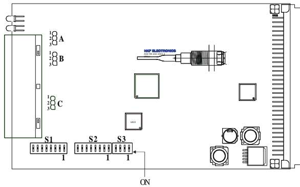
Figure 2. ADS TRA/B printed circuit board; details left out for clarity. Take care not to damage the optical fiber floating above the board.
