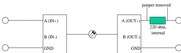
Figure 3. Current loop connections
