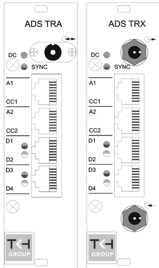
Figure 1. ADS front panels: TRA (left, similar to TRB, one-fiber), and TRX (right, two-fibers)
