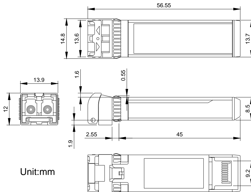
Figure 5. Outline Drawing
