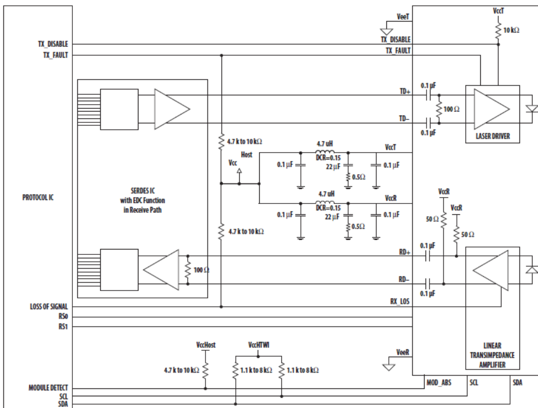
Figure 4. Recommended Application Interface Block Diagram
