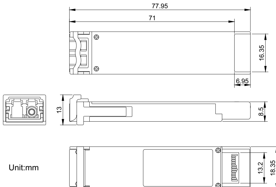
Figure 4. Outline Drawing
