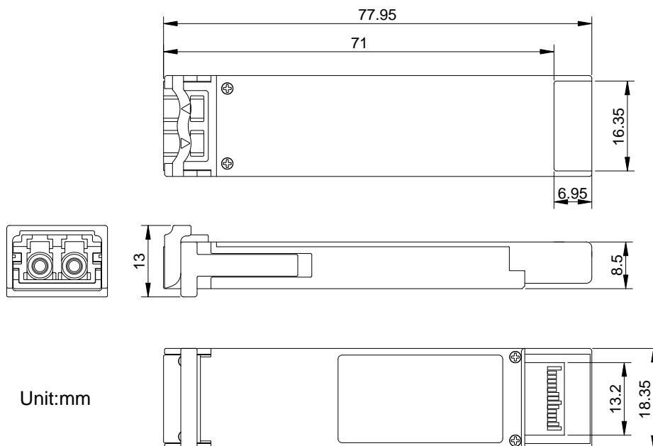
Figure 4. Outline Drawing
