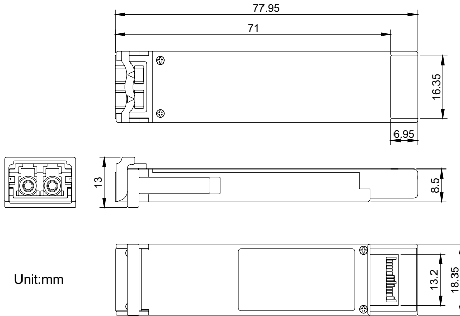
Figure 4. Outline Drawing
