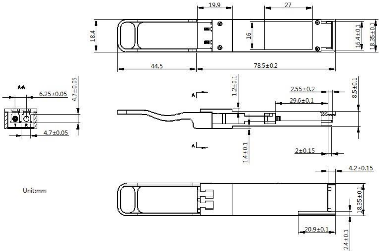
Figure 5. Outline Drawing
